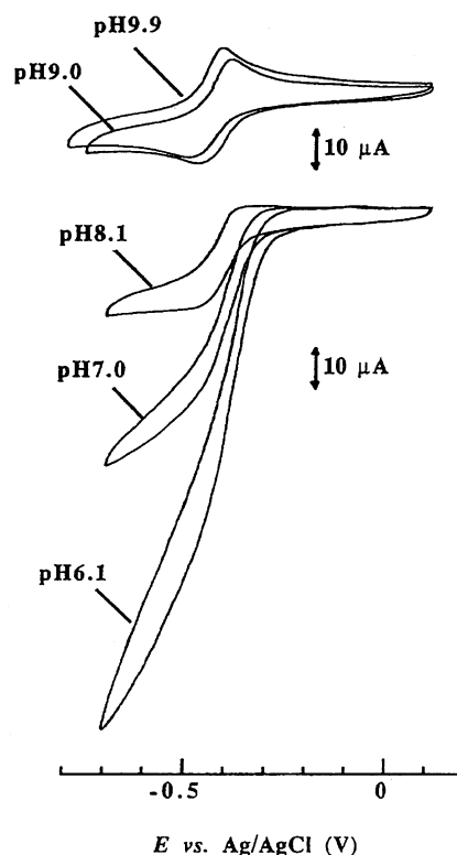
Fig. 4. Cyclic voltammograms of [Cu(H 2 O)(tpa)](ClO 4 ) 2 (1.01 mmol dm -3 ) in the presence of NaNO 2 (13.8 mmol dm -3 ) in H 2 O at various pH.
